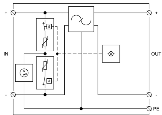
Internal diagram
